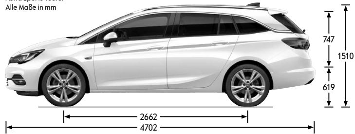
Astra Sports Tourer Alle Maße in mm
