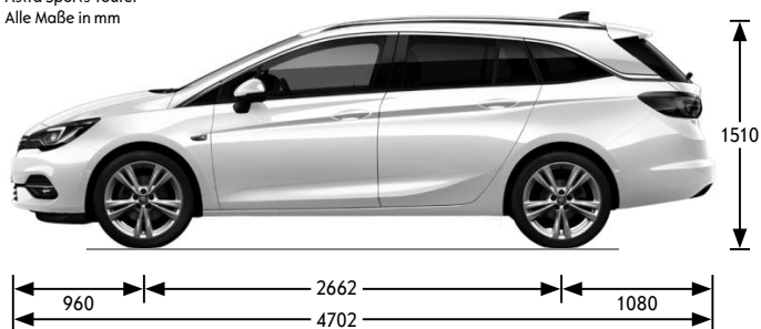
Astra Sports Tourer Alle Maße in mm
