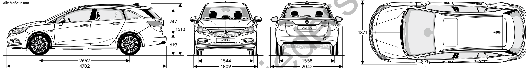
Astra Sports Tourer Alle Maße in mm
